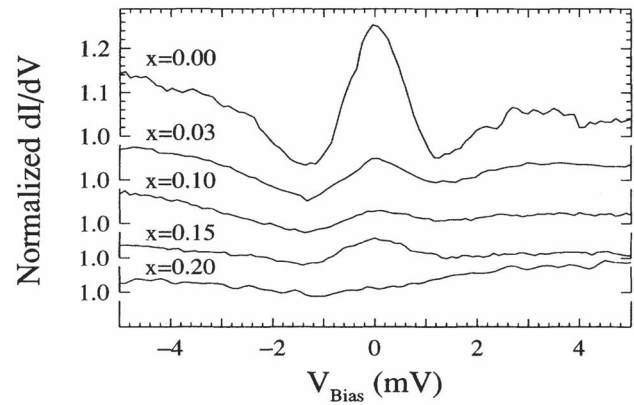
FIG. 42. Tunneling conductance spectra acquired at the vortex-core center of \text{Nb}_{1-x}\text{Ta}_x\text{Se}_2 at T=1.3 K and H=0.3 T for different impurity dopings x . For x=0 (clean limit), bound states are observed as a broad ZBCP, which progressively vanishes for larger amounts of impurities (Renner et al. , 1991).
