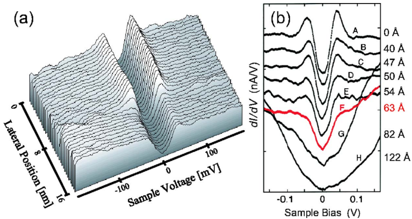
FIG. 31. (Color online) Pseudogap on disordered Bi2212 surfaces. (a) LDOS as a function of tip position on a Bi2212 300-Å-thick film at 4.2 K. Spectra were acquired every 5 Å. From Cren et al. , 2000 . (b) LDOS evolution through a locally damaged Bi2212 region. The values on the right indicate the distance of each spectrum relative to spectrum A. Adapted from Howald et al. , 2001 .
