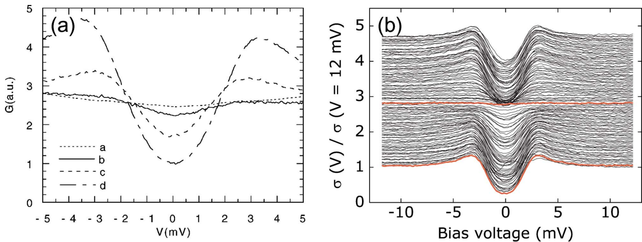
FIG. 43. (Color online) Examples of missing zero-bias peak in the vortex cores of conventional BCS superconductors. (a) Spectra acquired at 47 nm (dashed line) to the center of the core (dotted line) in \text{LuNi}_2\text{B}_2\text{C} at T=4.2 K and H=1.5 T. From DeWilde, Iavarone, Welp, Metlushko, Koshelev, Aranson, Crabtree, and Canfield, 1997. (b) 250-nm-long spectroscopic trace crossing a single vortex core in \text{MgB}_2 at T=2 K and H=0.2 T. From Eskildsen et al. , 2002.
